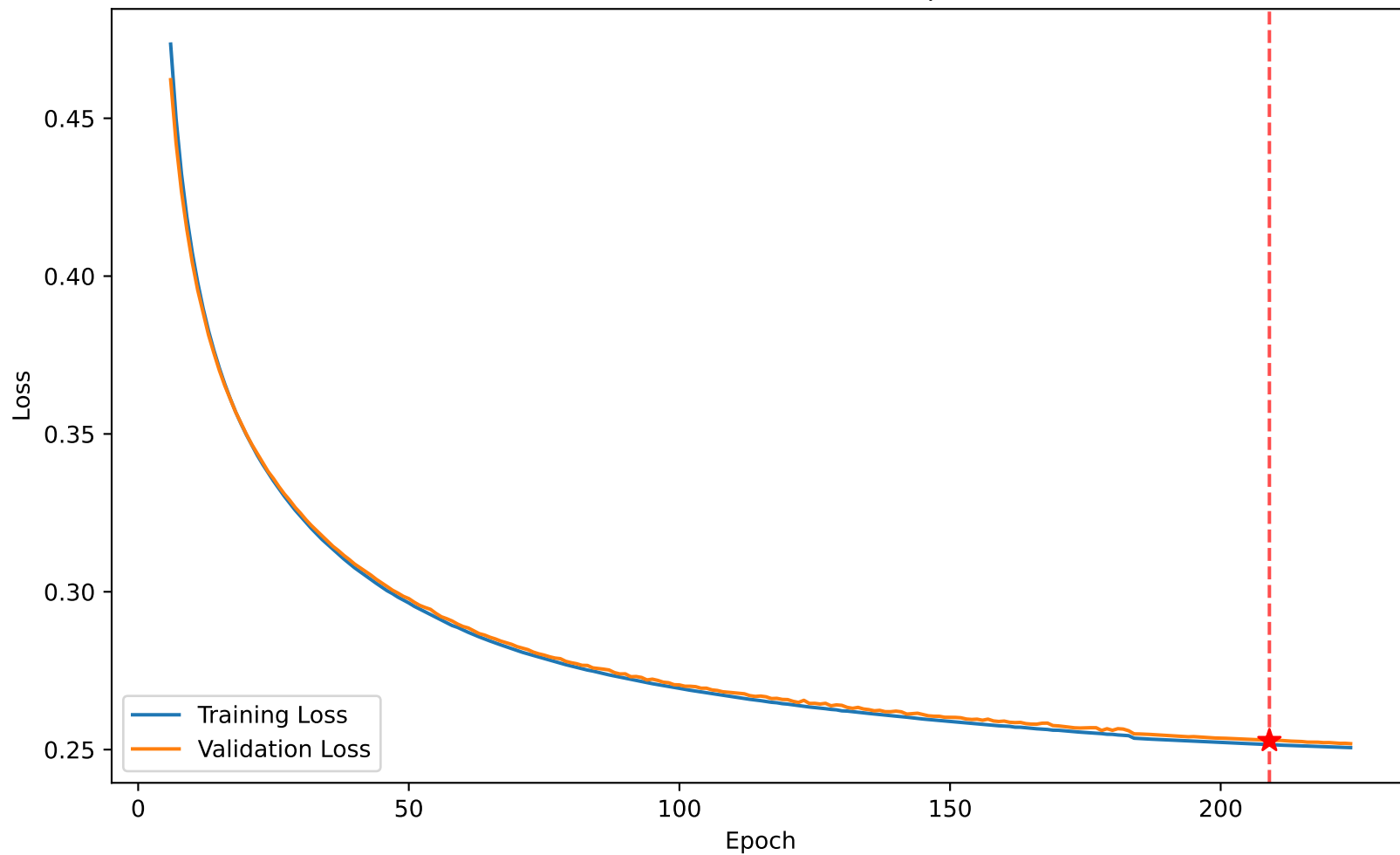
Loss 0.252 vs Val Loss 0.253 at epoch 209
