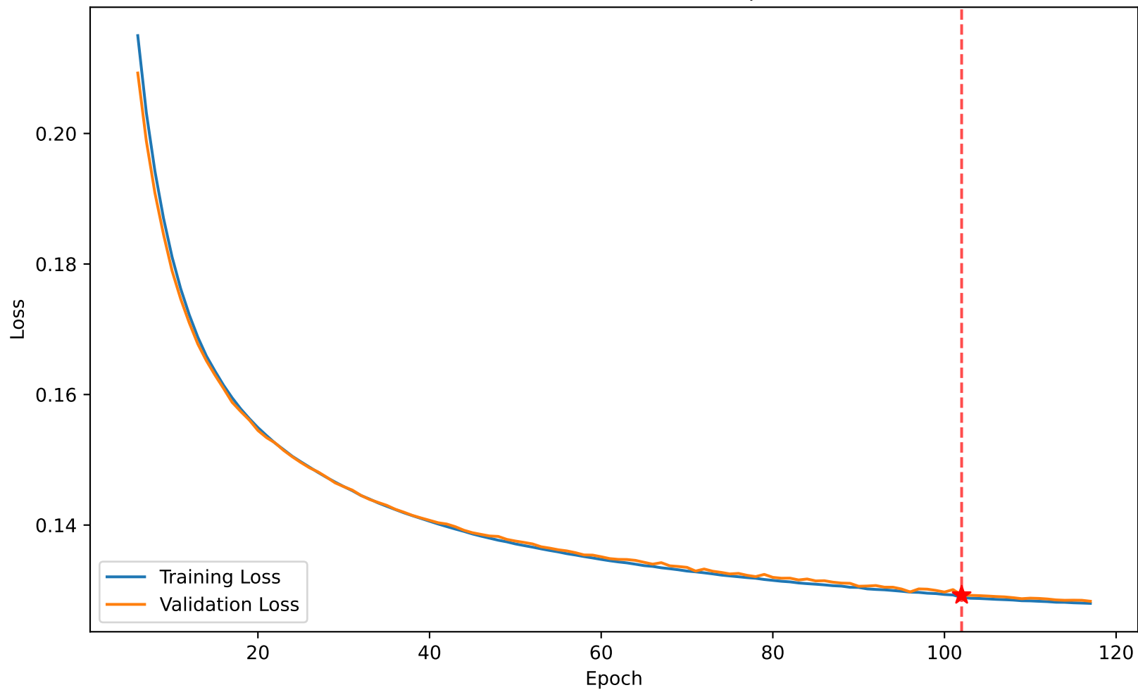
Loss 0.129 vs Val Loss 0.129 at epoch 102
