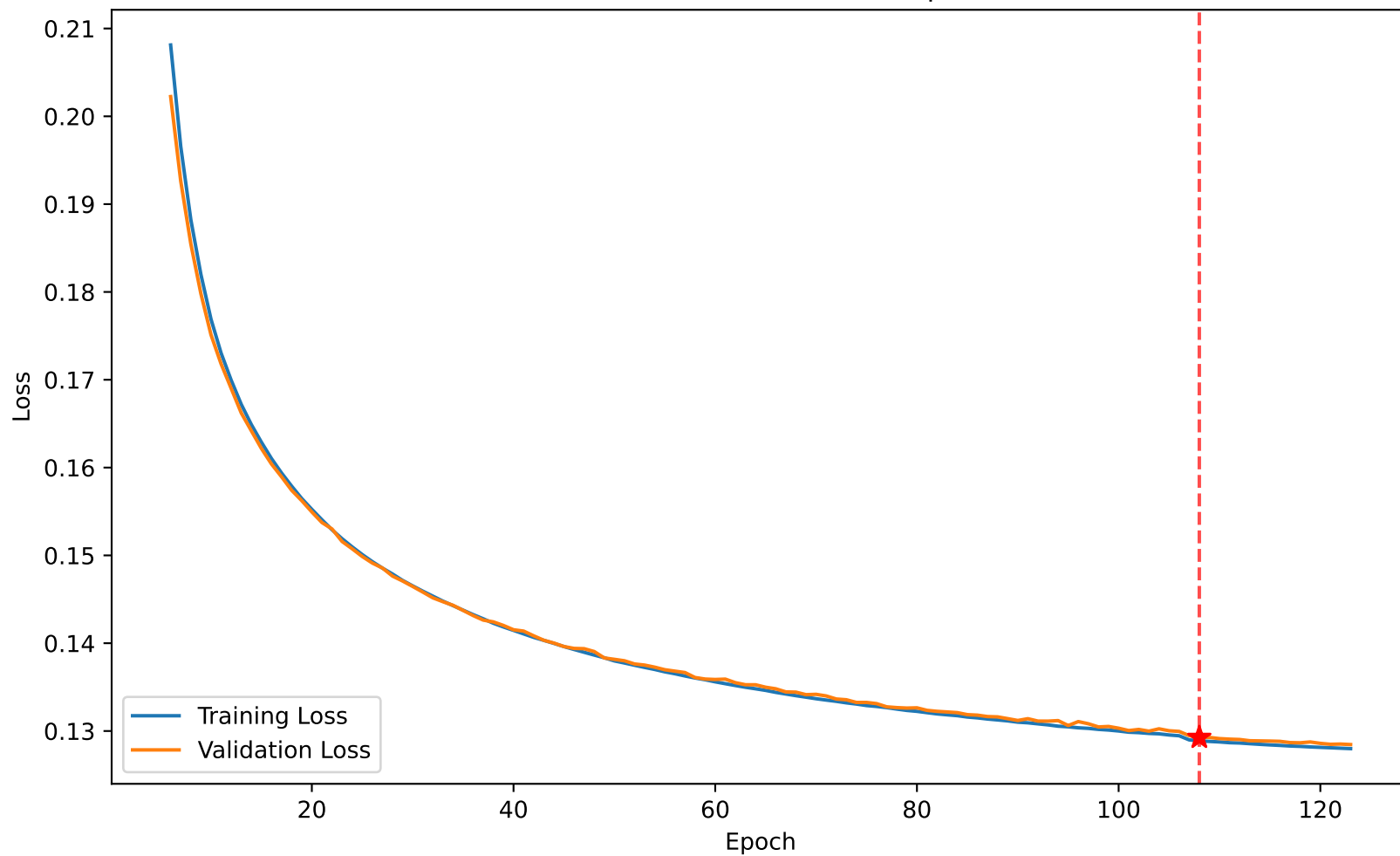
Loss 0.129 vs Val Loss 0.129 at epoch 108
