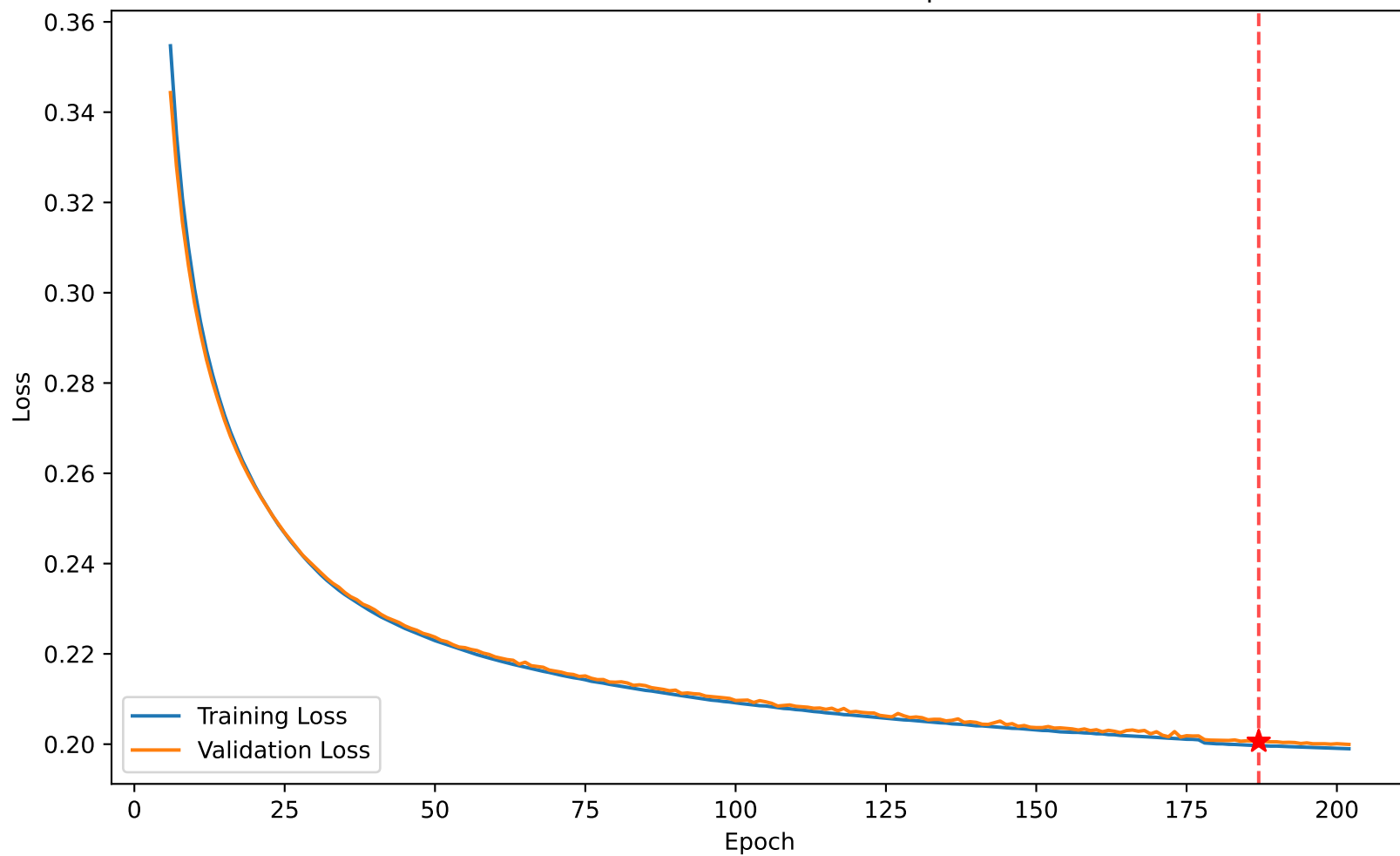
Loss 0.200 vs Val Loss 0.201 at epoch 187
