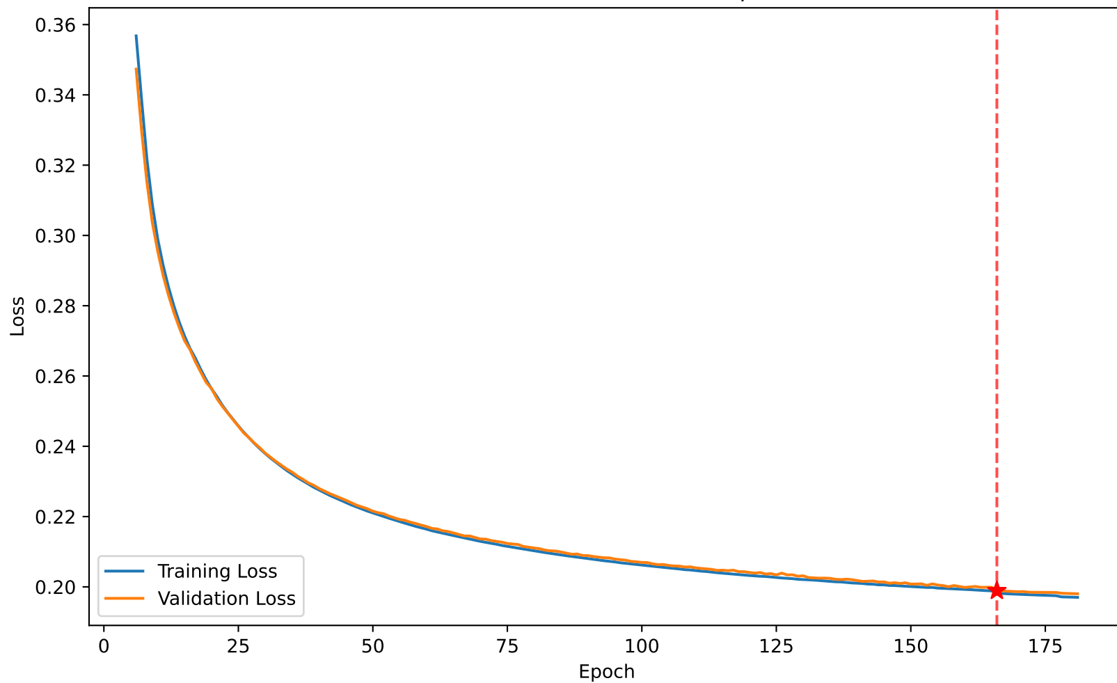
Loss 0.198 vs Val Loss 0.199 at epoch 166
