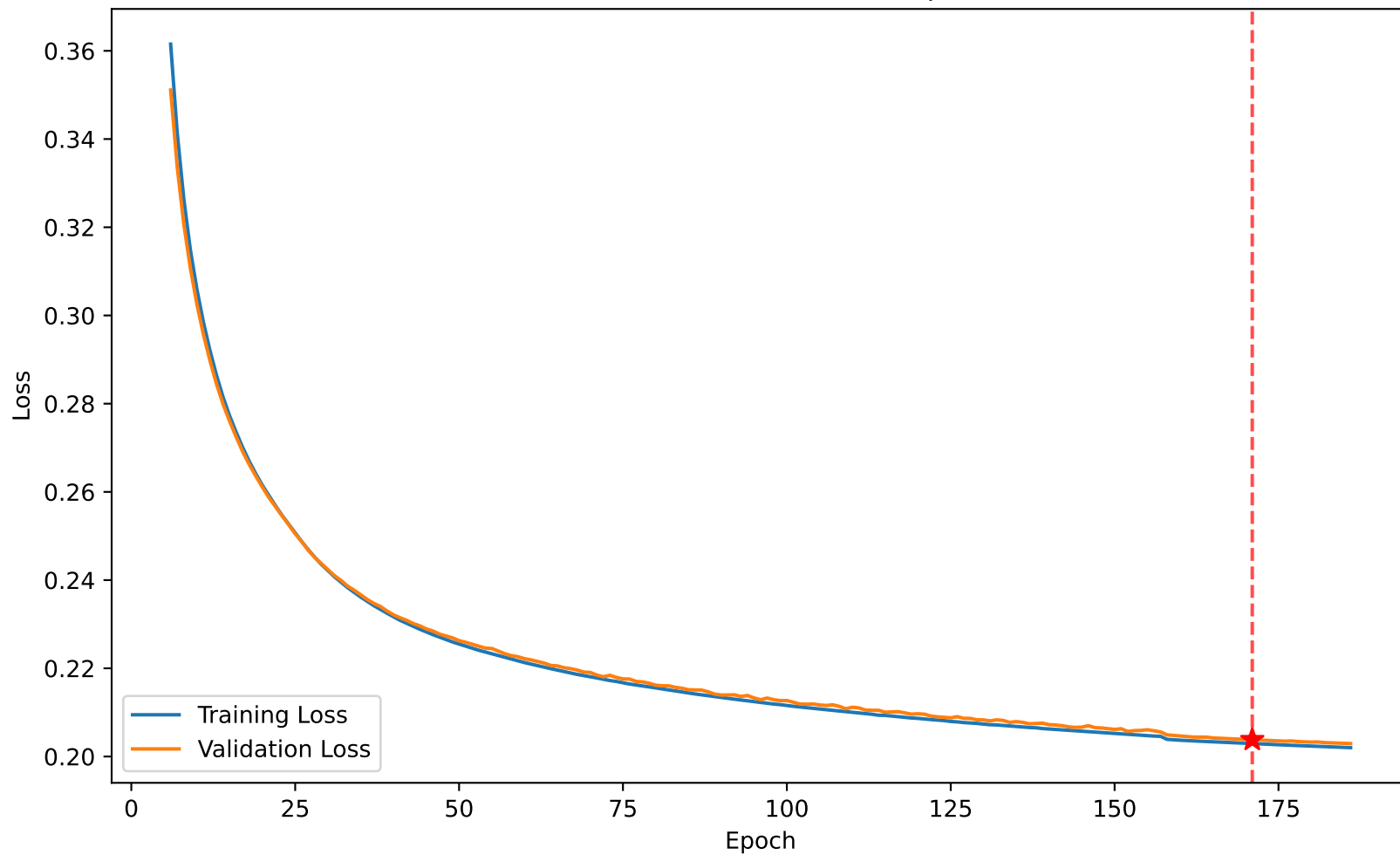
Loss 0.203 vs Val Loss 0.204 at epoch 171
