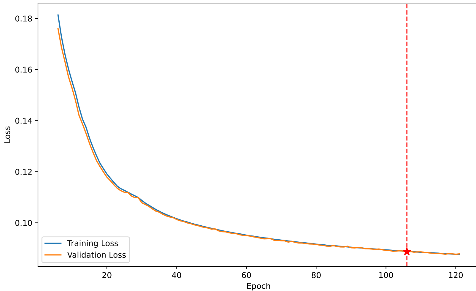
Loss 0.089 vs Val Loss 0.089 at epoch 106
