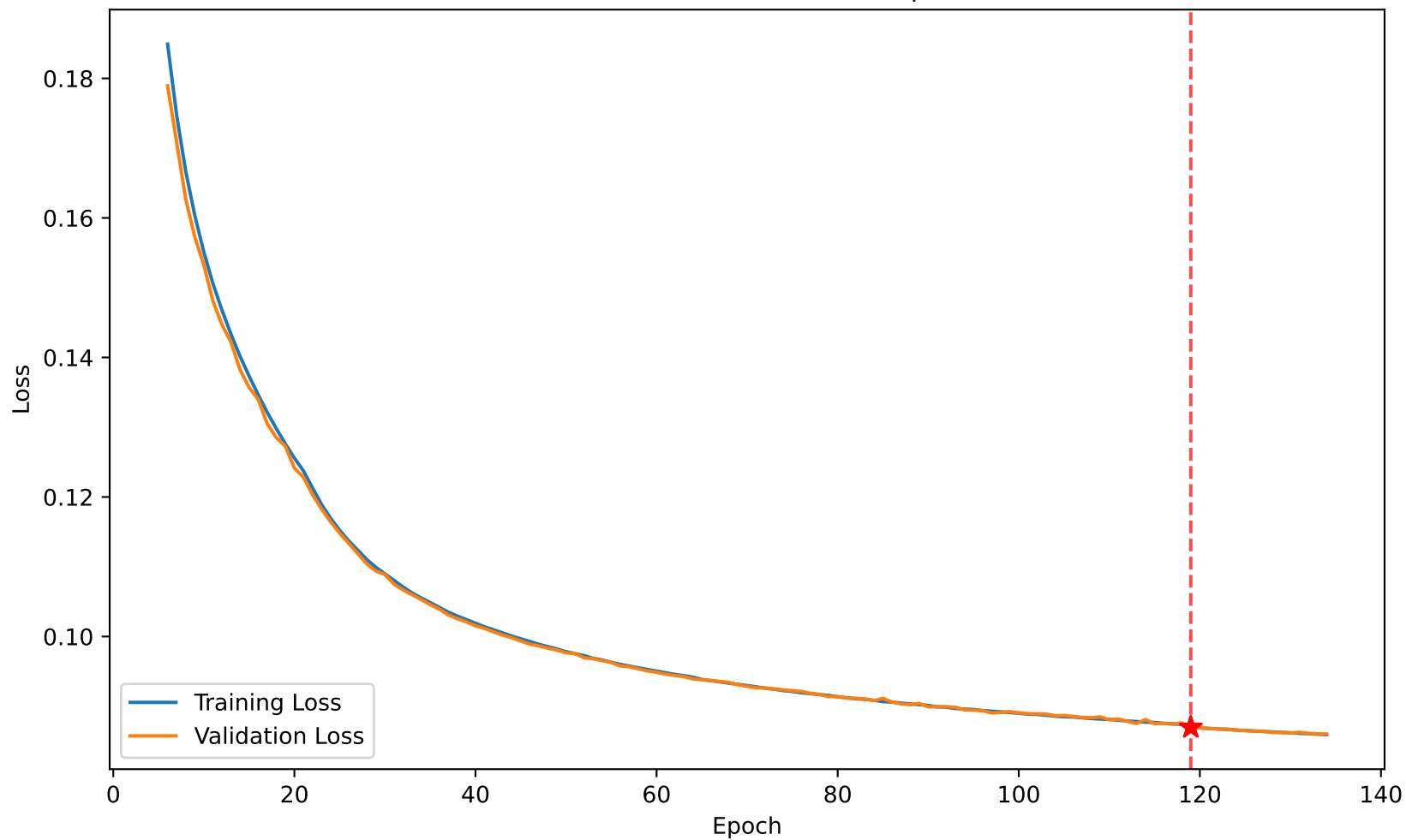
Loss 0.087 vs Val Loss 0.087 at epoch 119
