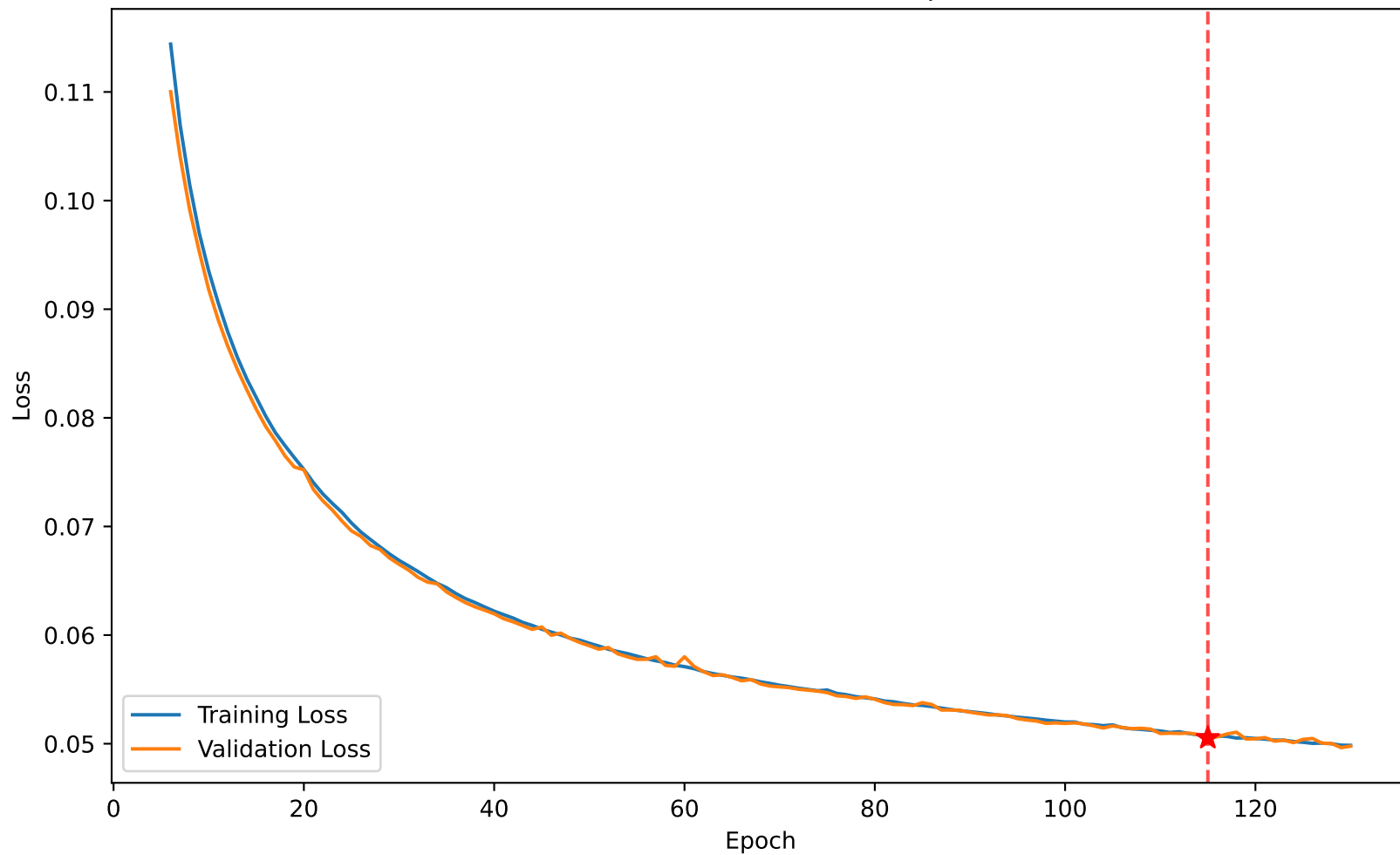
Loss 0.051 vs Val Loss 0.051 at epoch 115
