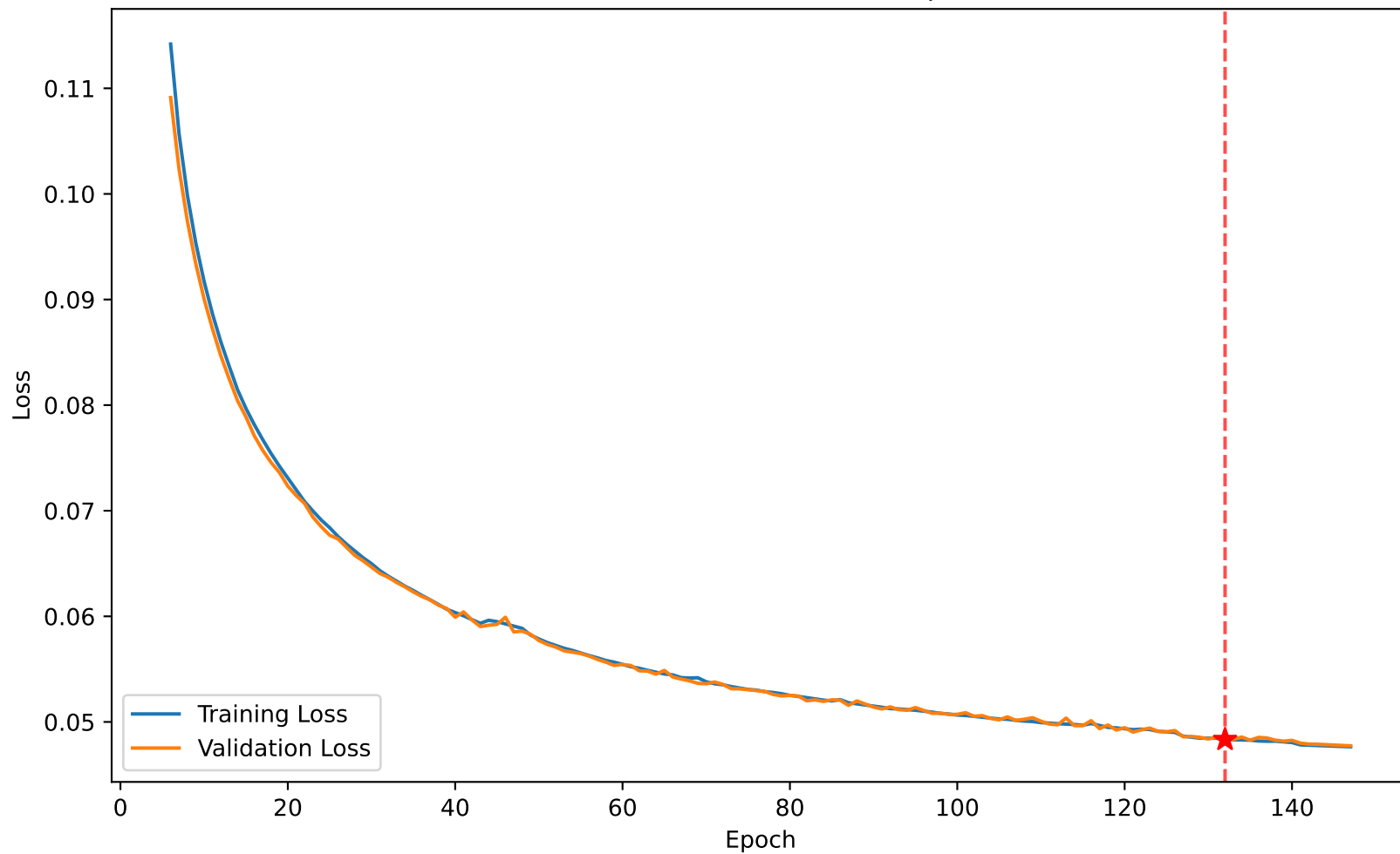
Loss 0.048 vs Val Loss 0.048 at epoch 132
