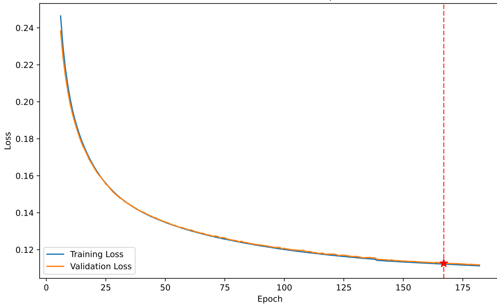
Loss 0.112 vs Val Loss 0.113 at epoch 167
