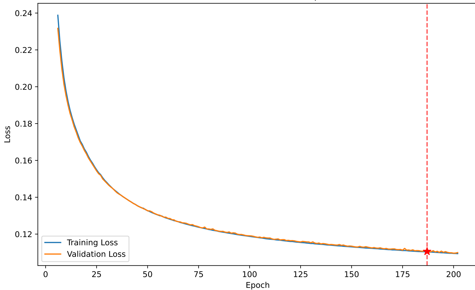
Loss 0.110 vs Val Loss 0.111 at epoch 187
