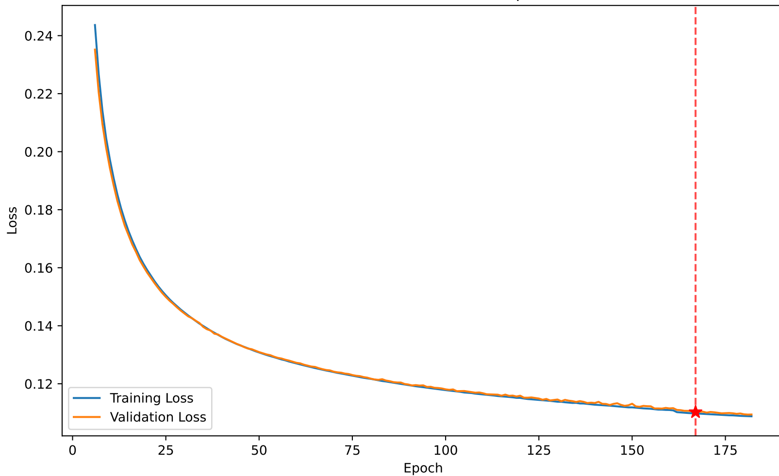
Loss 0.110 vs Val Loss 0.110 at epoch 167
