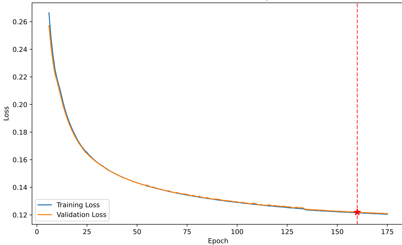
Loss 0.122 vs Val Loss 0.122 at epoch 160
