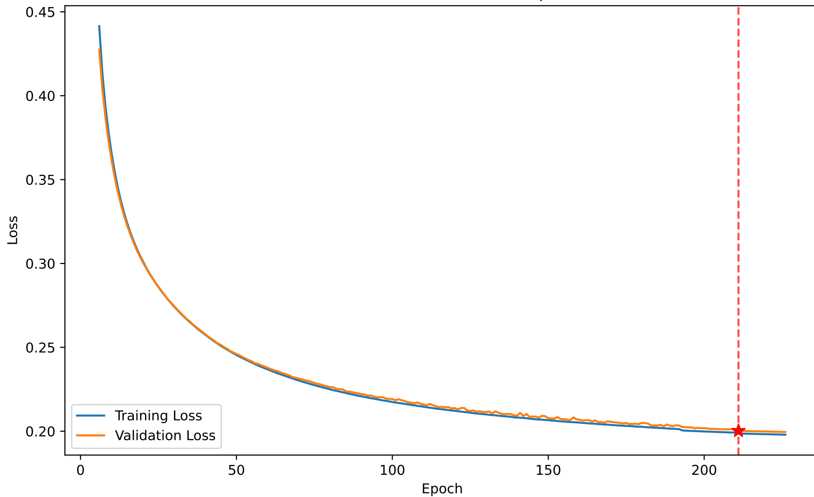
Loss 0.199 vs Val Loss 0.200 at epoch 211
