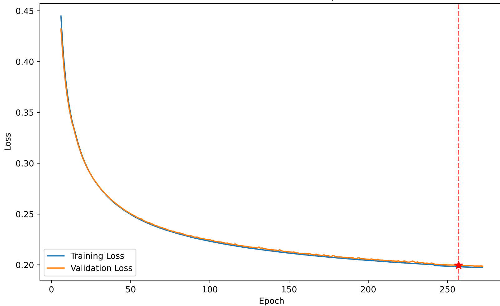
Loss 0.198 vs Val Loss 0.199 at epoch 257
