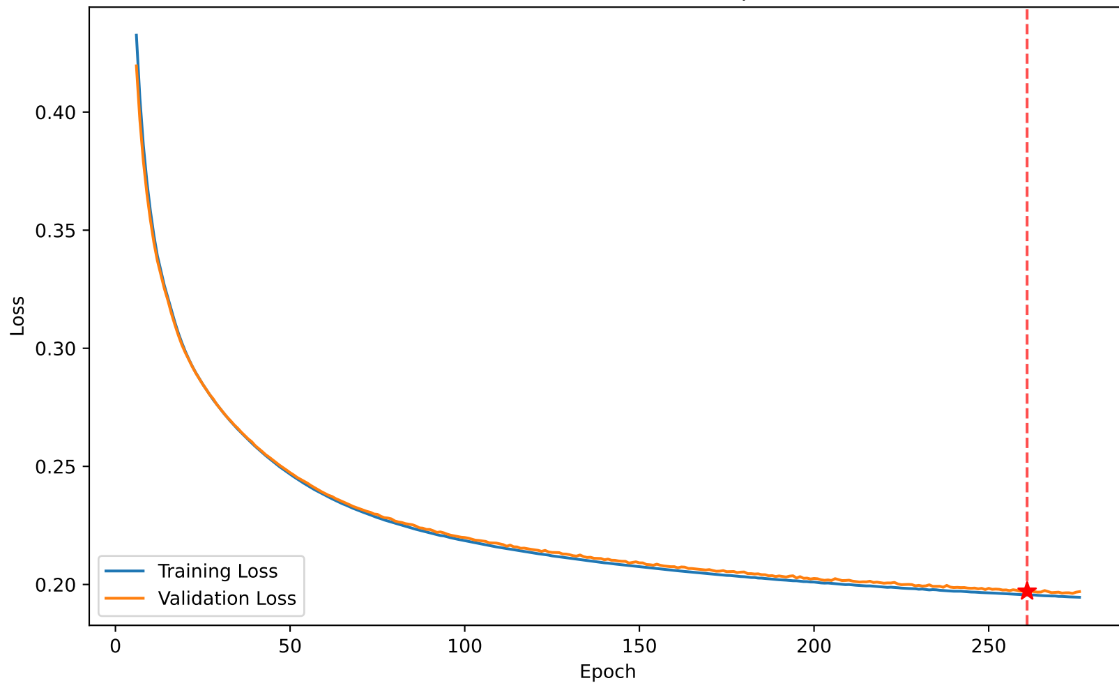
Loss 0.196 vs Val Loss 0.197 at epoch 261
