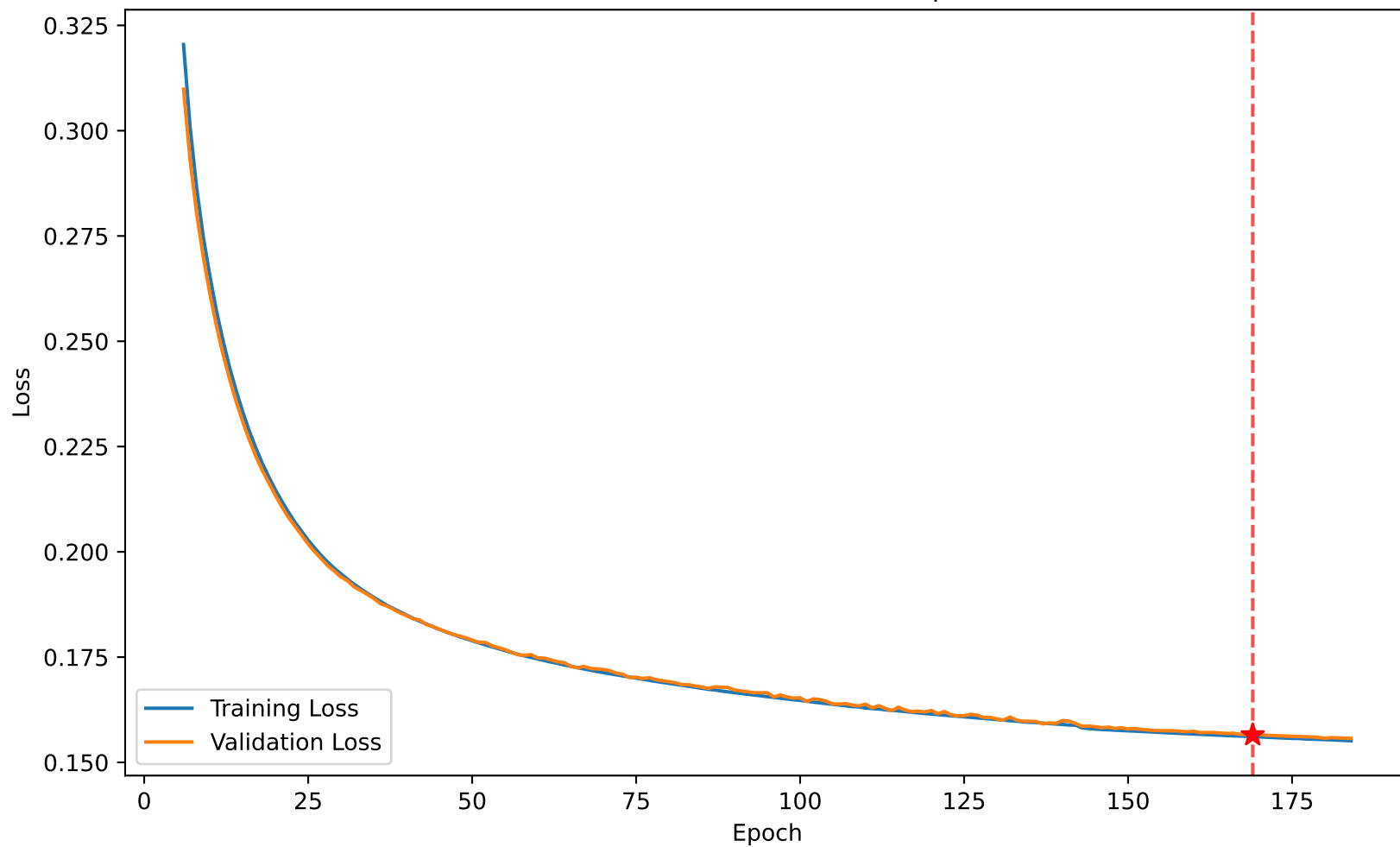
Loss 0.156 vs Val Loss 0.157 at epoch 169
