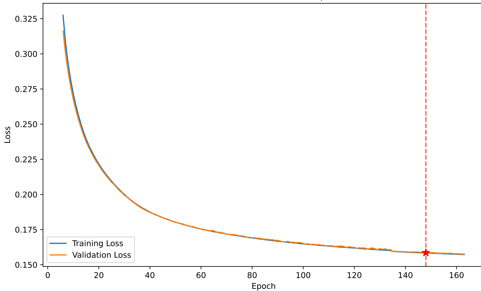
Loss 0.158 vs Val Loss 0.159 at epoch 148
