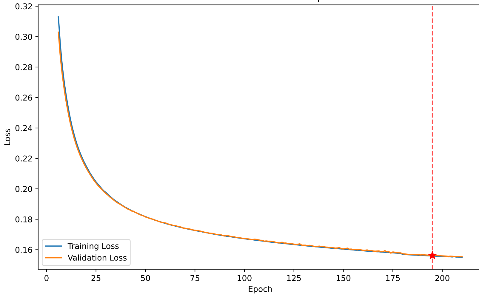
Loss 0.156 vs Val Loss 0.156 at epoch 195
