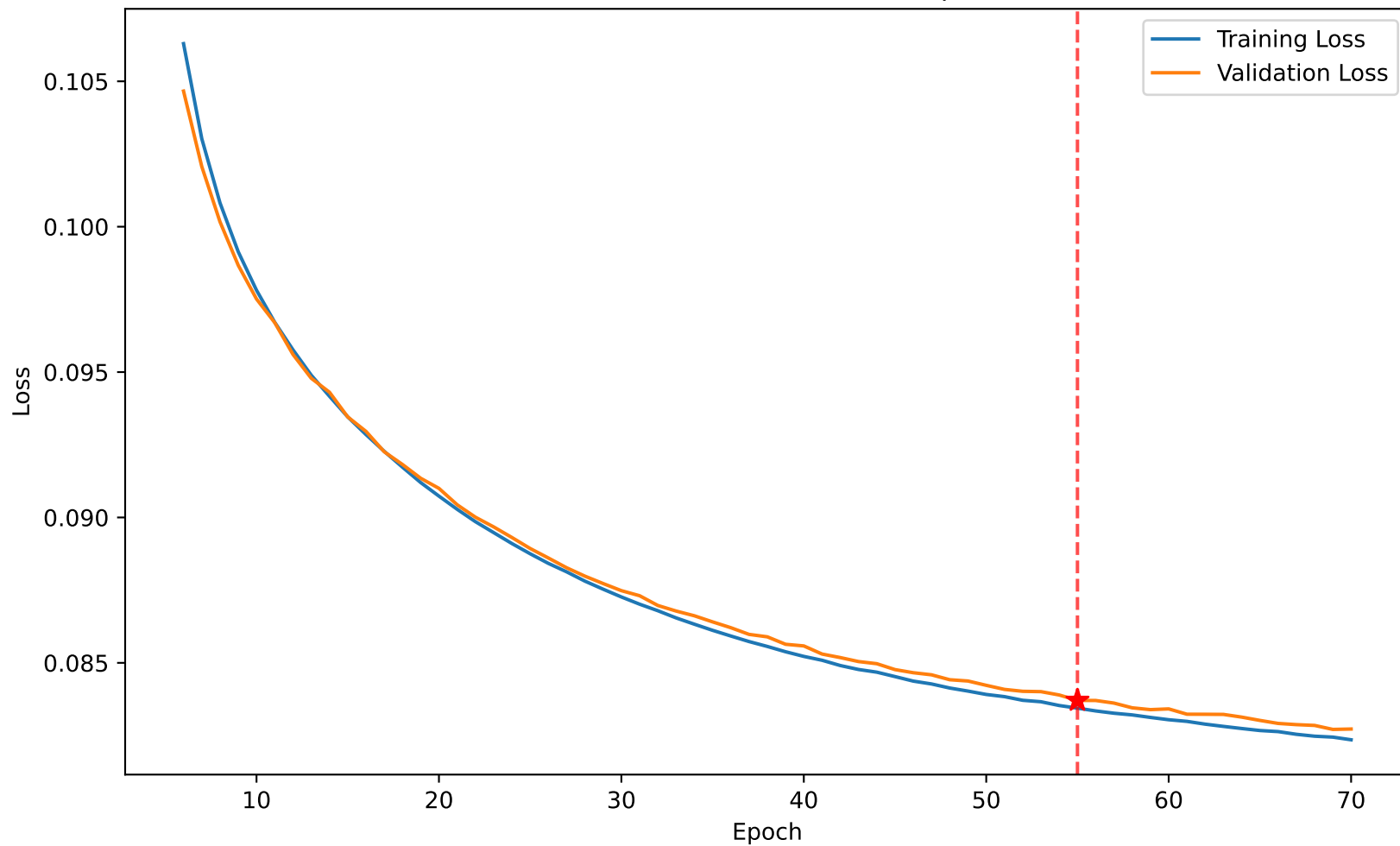
Loss 0.083 vs Val Loss 0.084 at epoch 55
