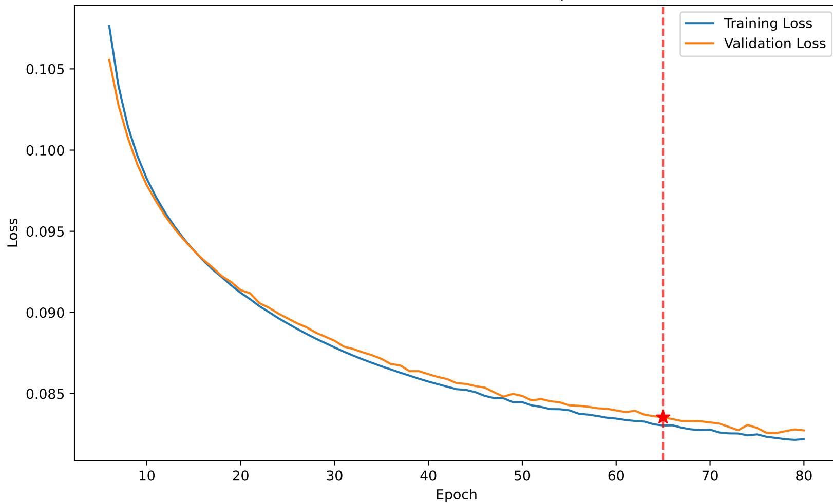
Loss 0.083 vs Val Loss 0.084 at epoch 65
