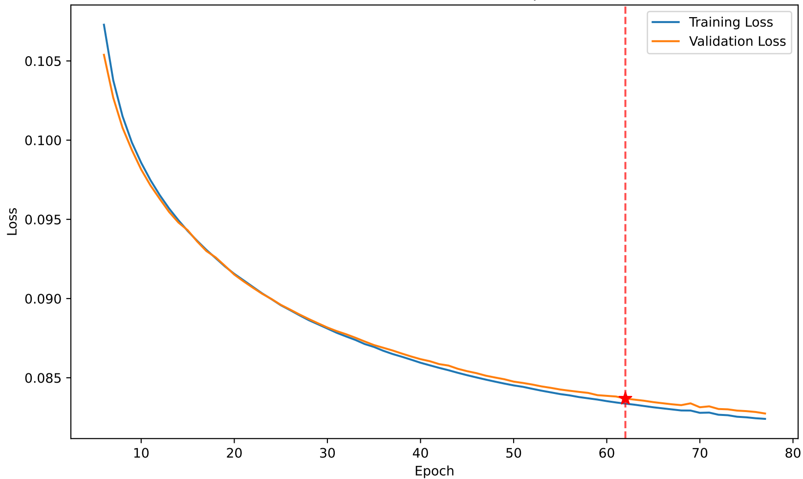
Loss 0.083 vs Val Loss 0.084 at epoch 62
