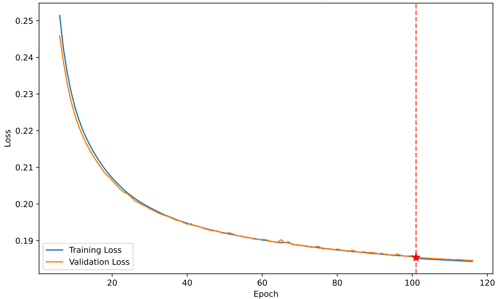
Loss 0.185 vs Val Loss 0.185 at epoch 101
