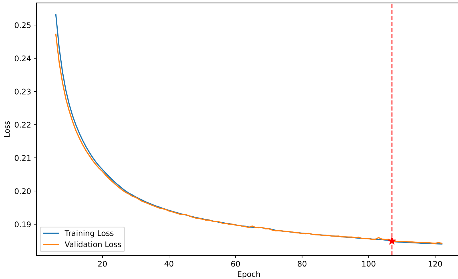
Loss 0.185 vs Val Loss 0.185 at epoch 107
