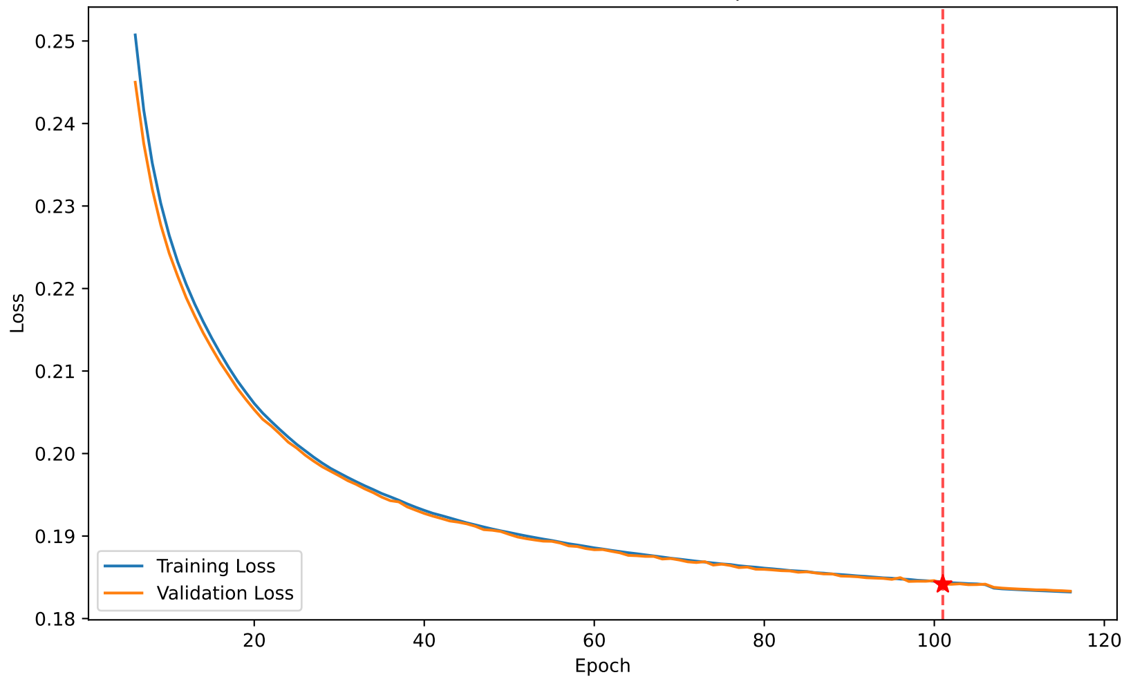
Loss 0.184 vs Val Loss 0.184 at epoch 101
