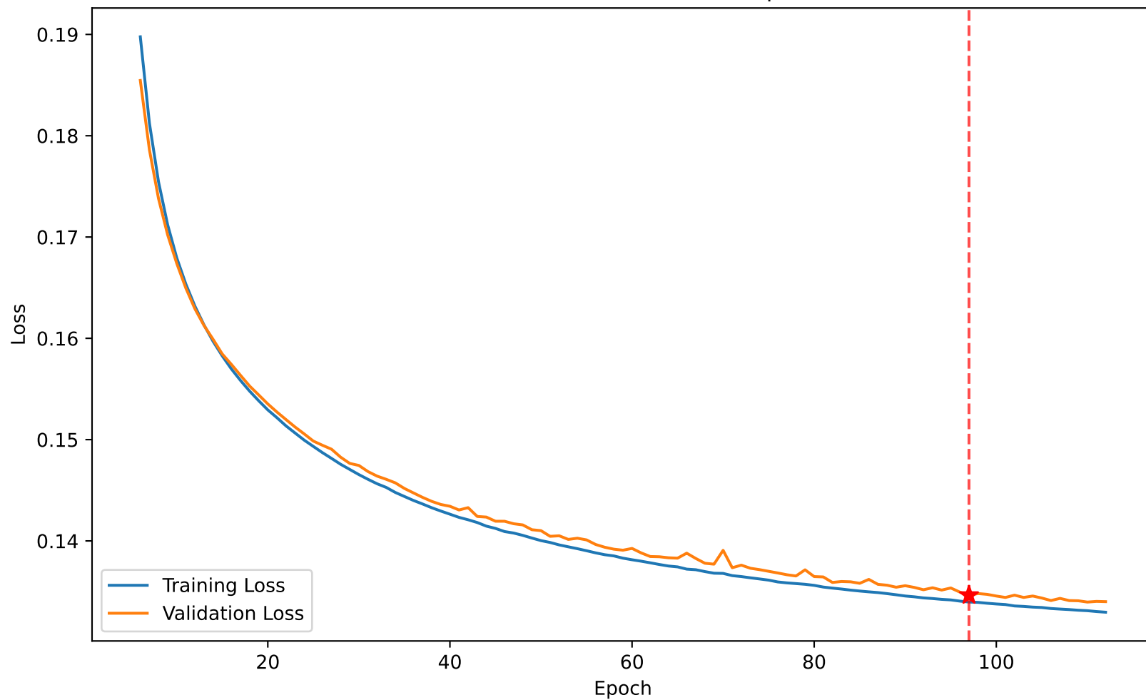
Loss 0.134 vs Val Loss 0.135 at epoch 97
