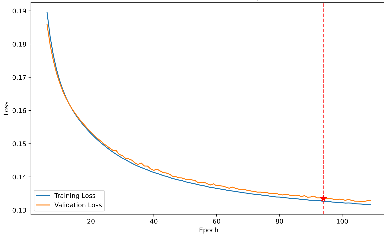
Loss 0.133 vs Val Loss 0.134 at epoch 94
