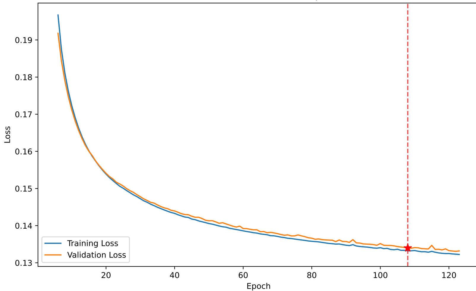
Loss 0.133 vs Val Loss 0.134 at epoch 108
