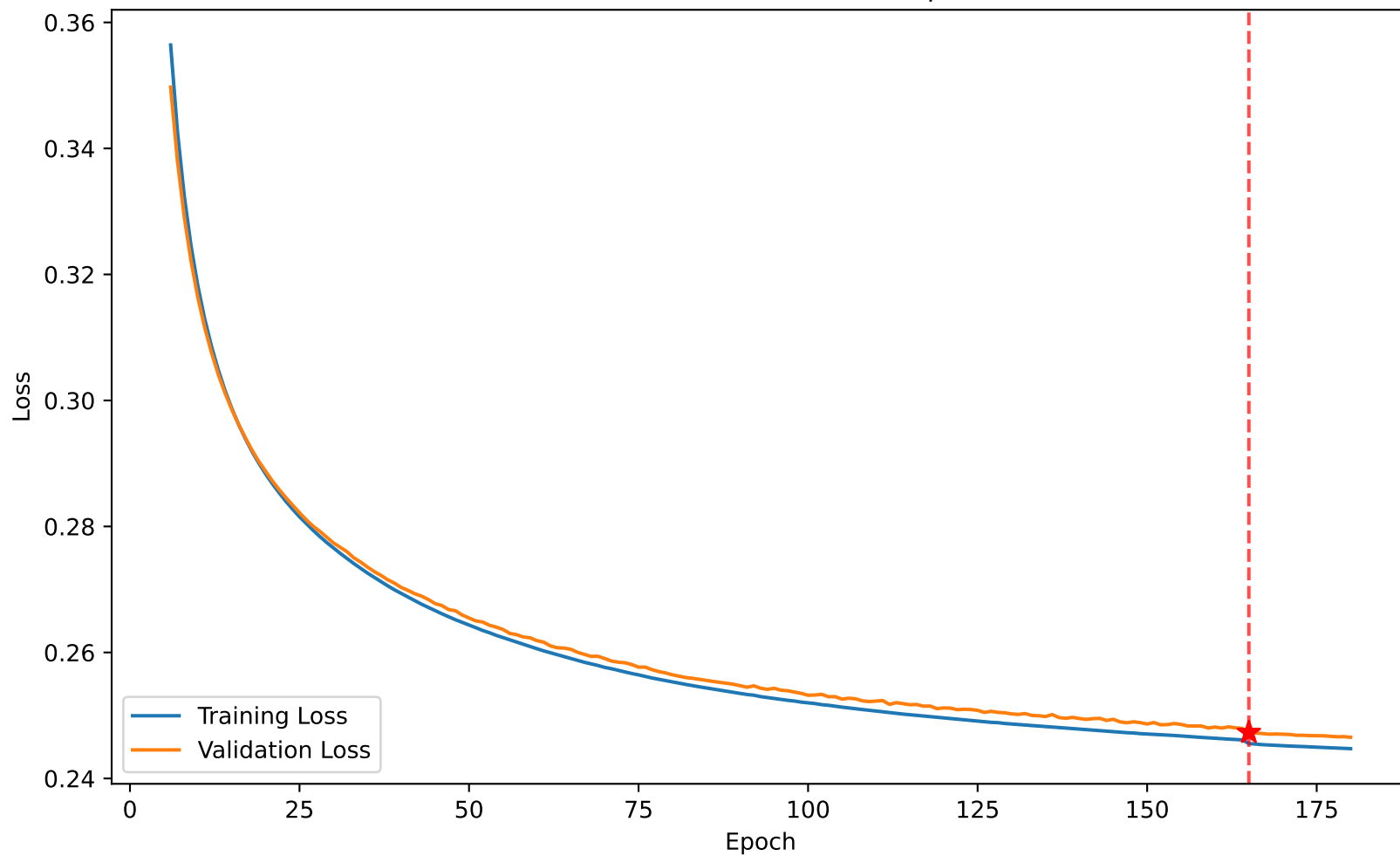
Loss 0.246 vs Val Loss 0.247 at epoch 165
