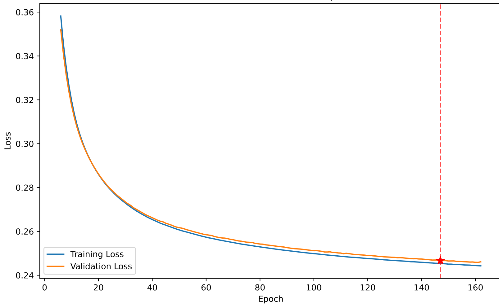
Loss 0.245 vs Val Loss 0.247 at epoch 147
