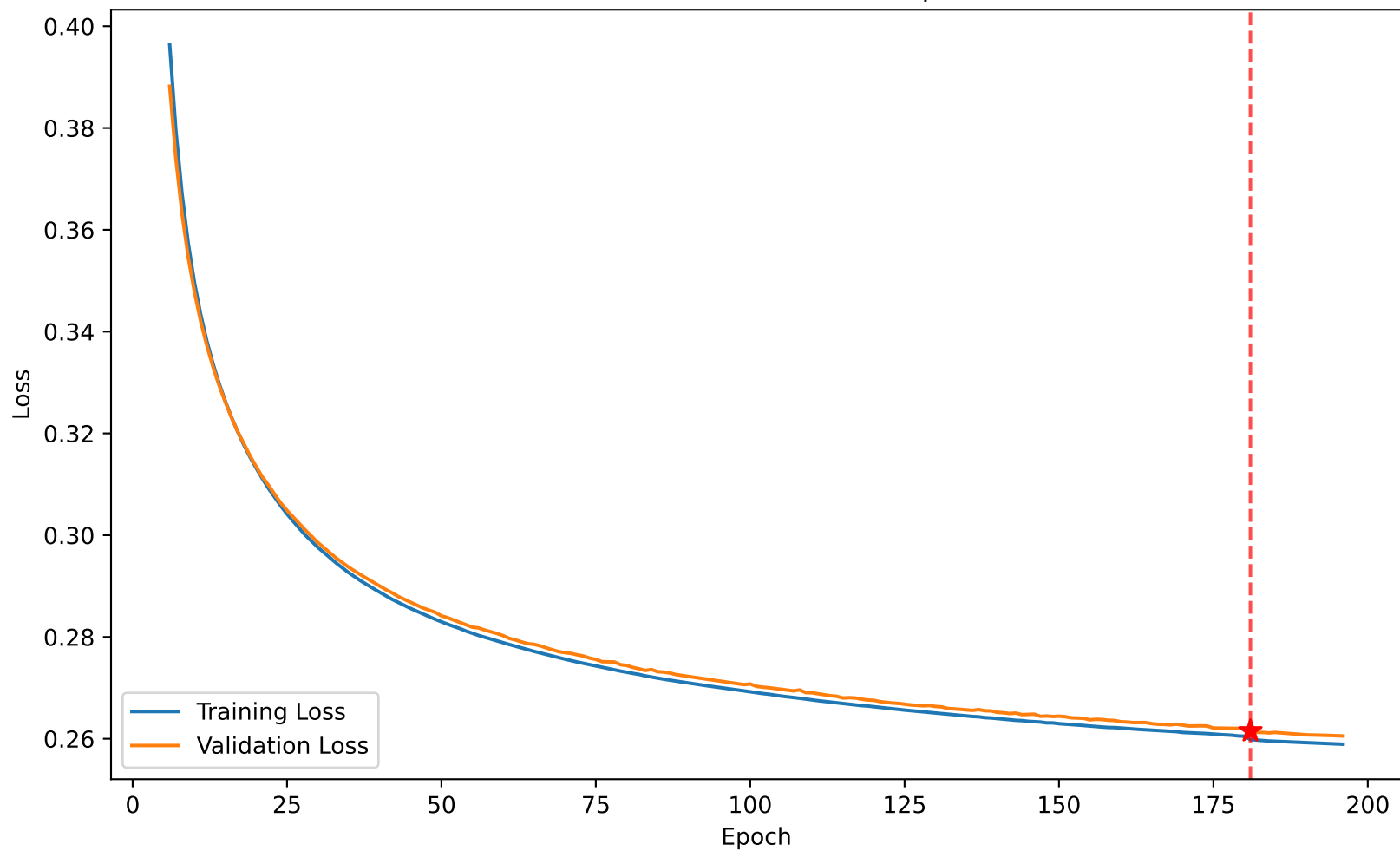
Loss 0.260 vs Val Loss 0.262 at epoch 181
