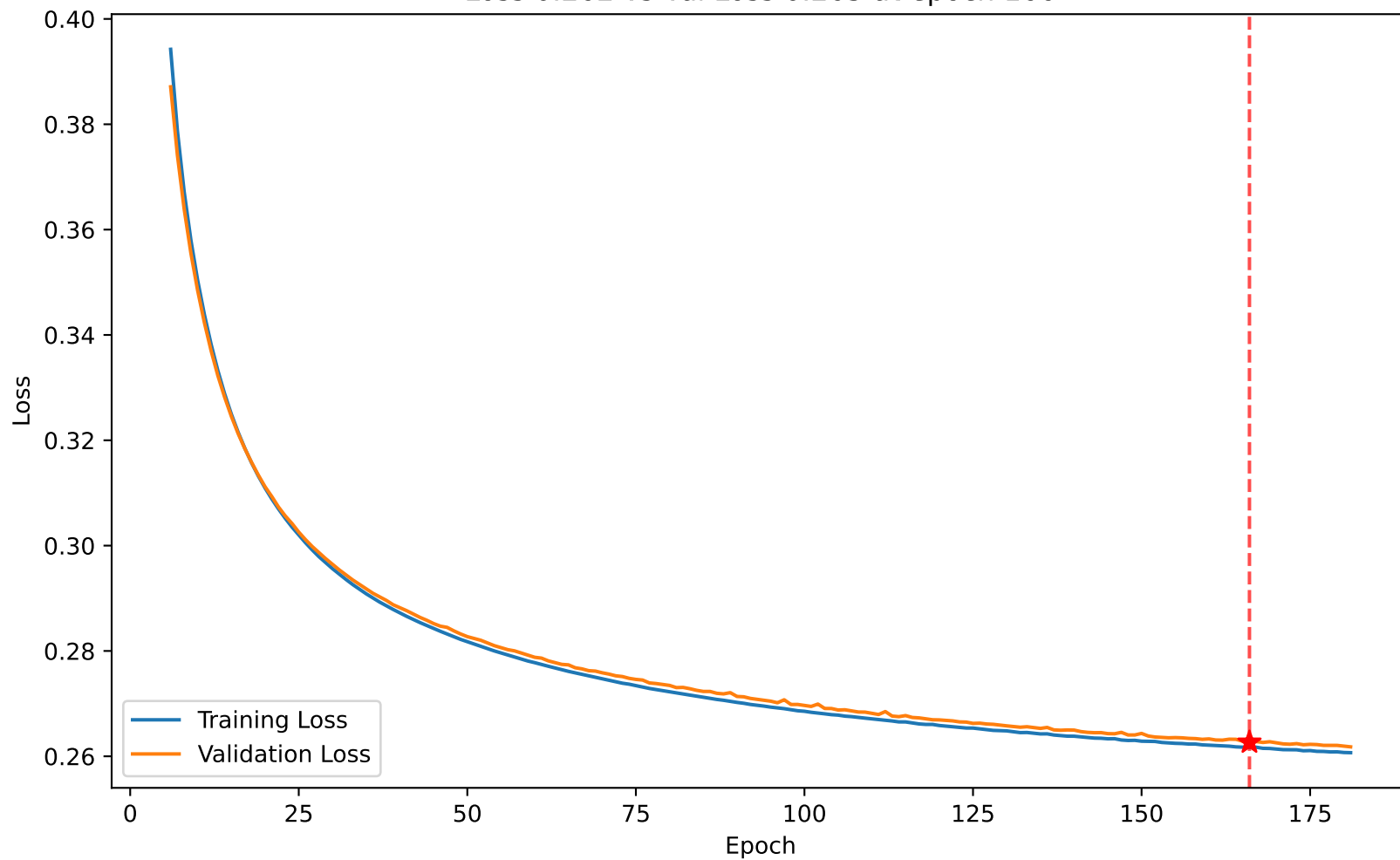
Loss 0.262 vs Val Loss 0.263 at epoch 166
