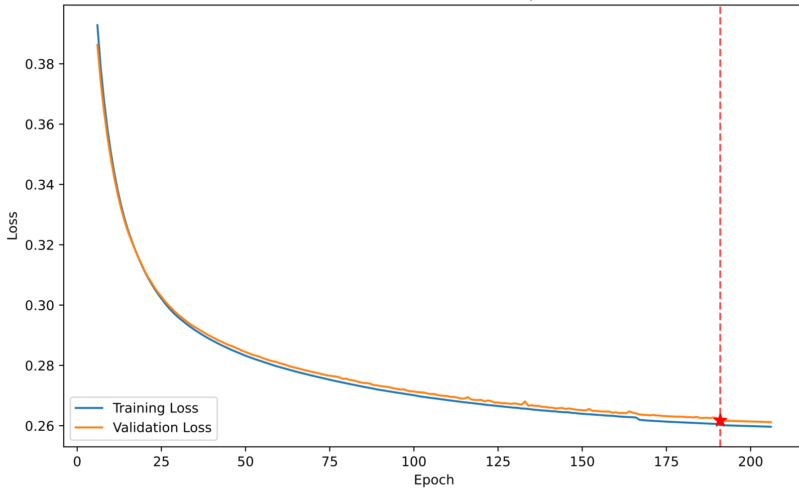
Loss 0.260 vs Val Loss 0.262 at epoch 191
