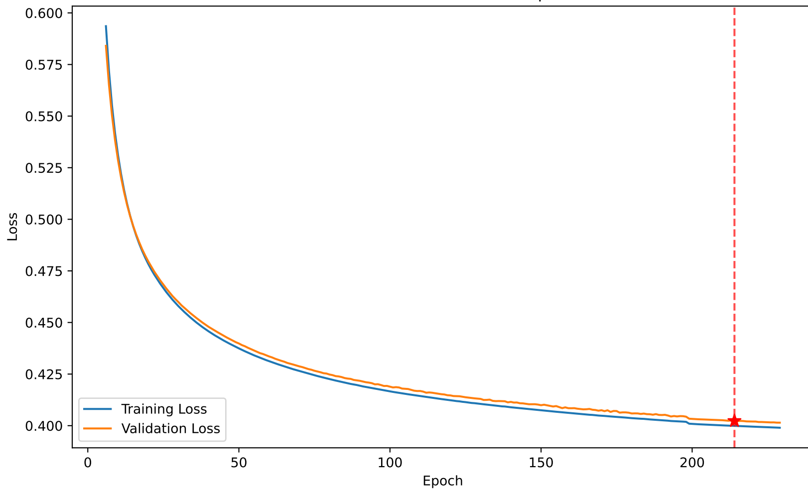
Loss 0.400 vs Val Loss 0.402 at epoch 214
