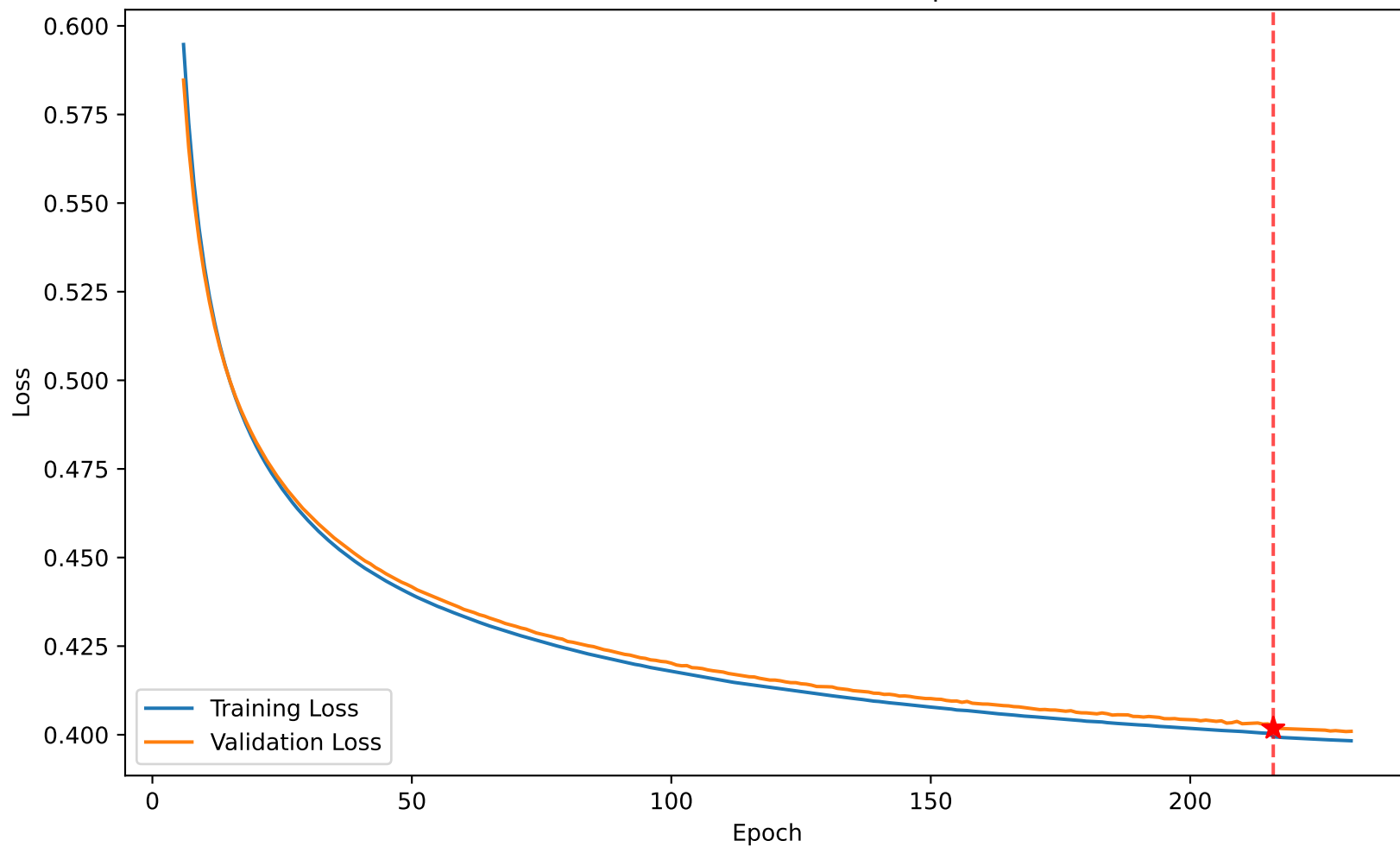
Loss 0.399 vs Val Loss 0.402 at epoch 216
