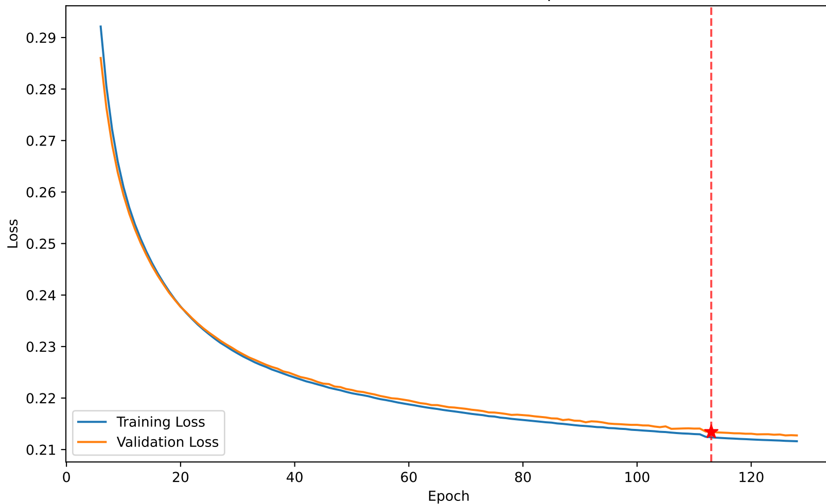
Loss 0.212 vs Val Loss 0.213 at epoch 113
