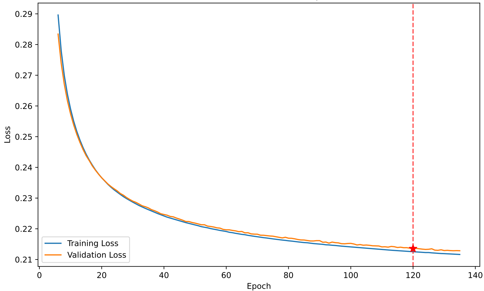
Loss 0.213 vs Val Loss 0.214 at epoch 120
