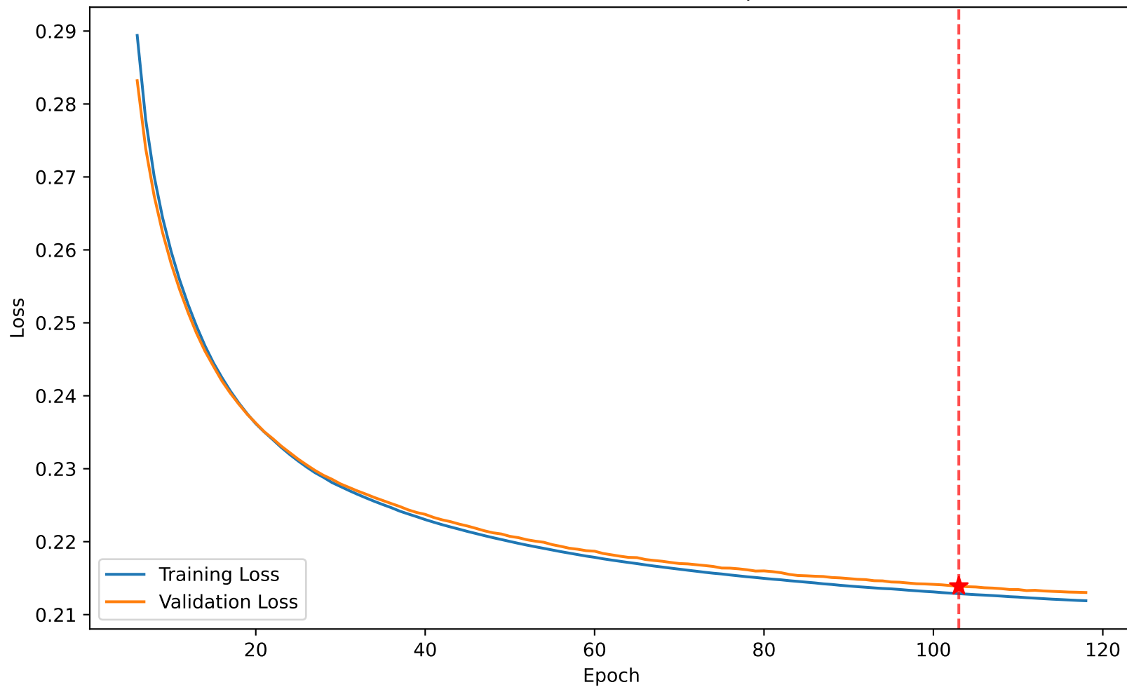
Loss 0.213 vs Val Loss 0.214 at epoch 103
