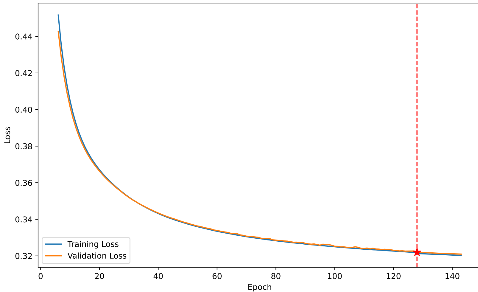
Loss 0.321 vs Val Loss 0.322 at epoch 128
