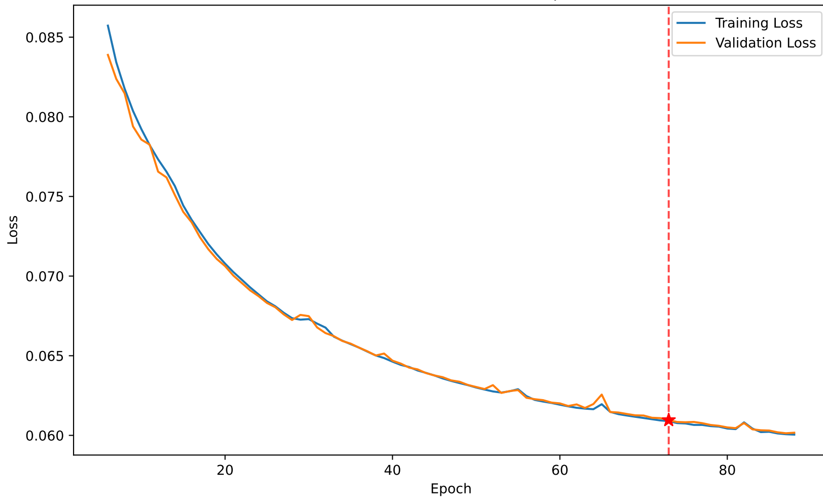
Loss 0.061 vs Val Loss 0.061 at epoch 73
