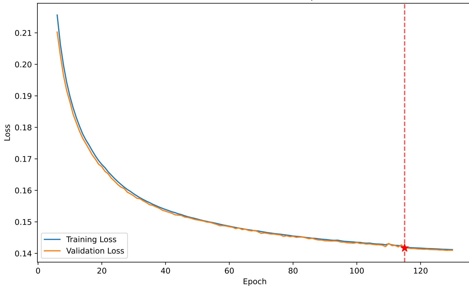
Loss 0.142 vs Val Loss 0.142 at epoch 115
