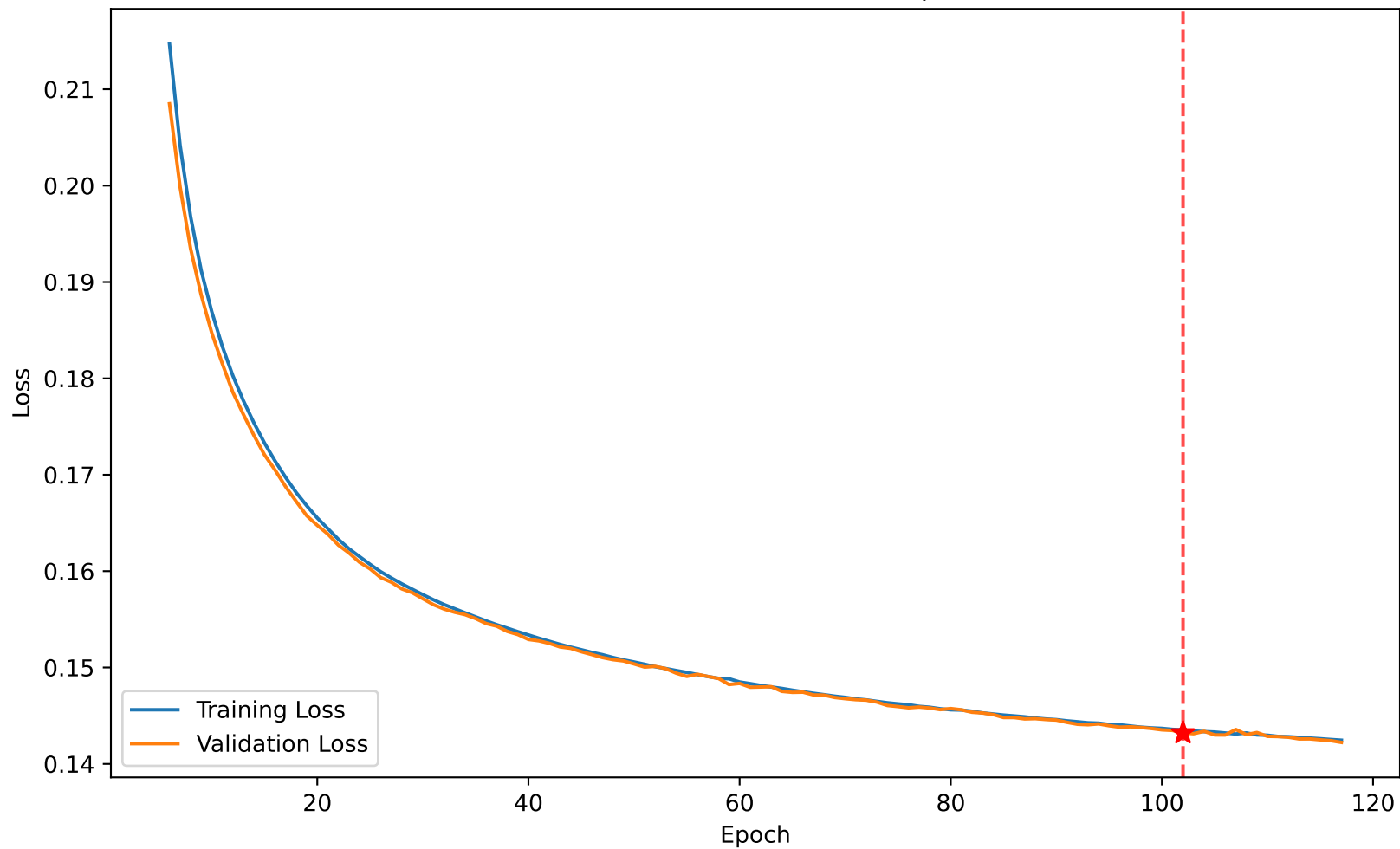
Loss 0.144 vs Val Loss 0.143 at epoch 102
