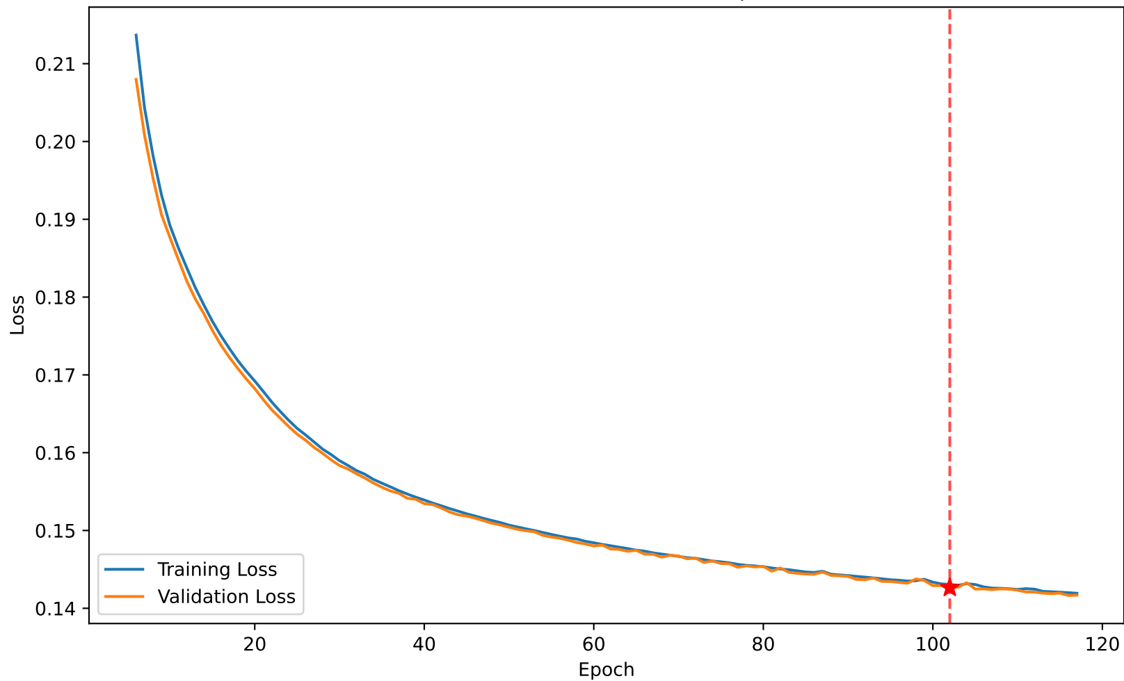
Loss 0.143 vs Val Loss 0.143 at epoch 102
