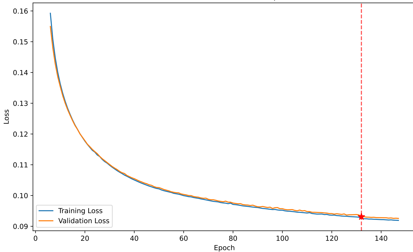
Loss 0.093 vs Val Loss 0.093 at epoch 132
