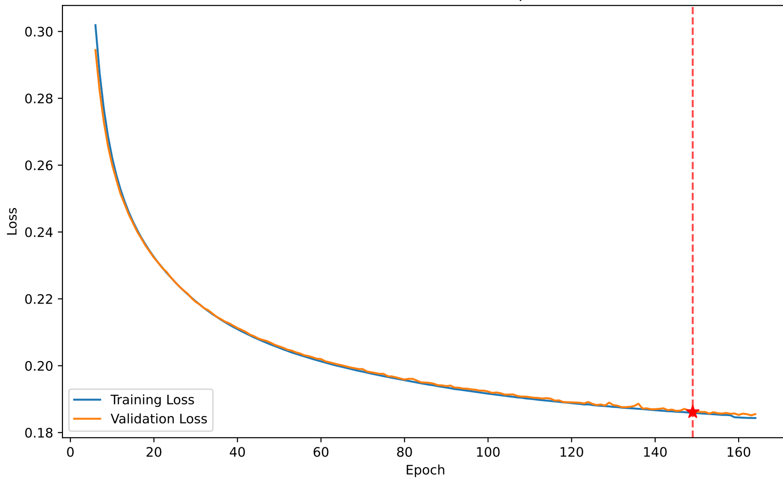
Loss 0.186 vs Val Loss 0.186 at epoch 149
