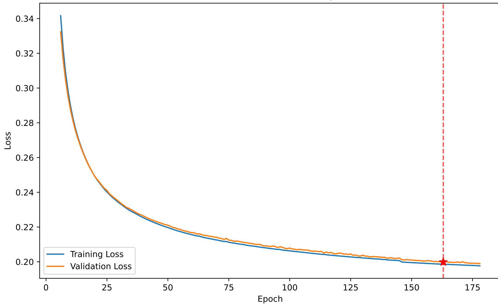
Loss 0.199 vs Val Loss 0.200 at epoch 163
