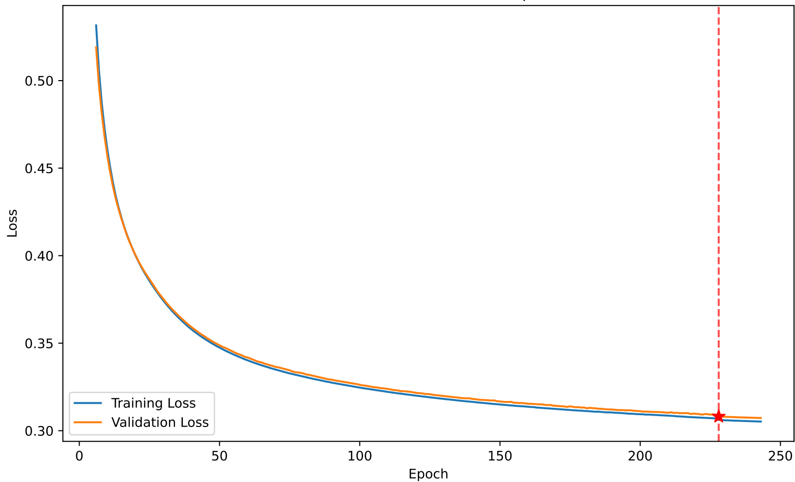
Loss 0.306 vs Val Loss 0.308 at epoch 228
