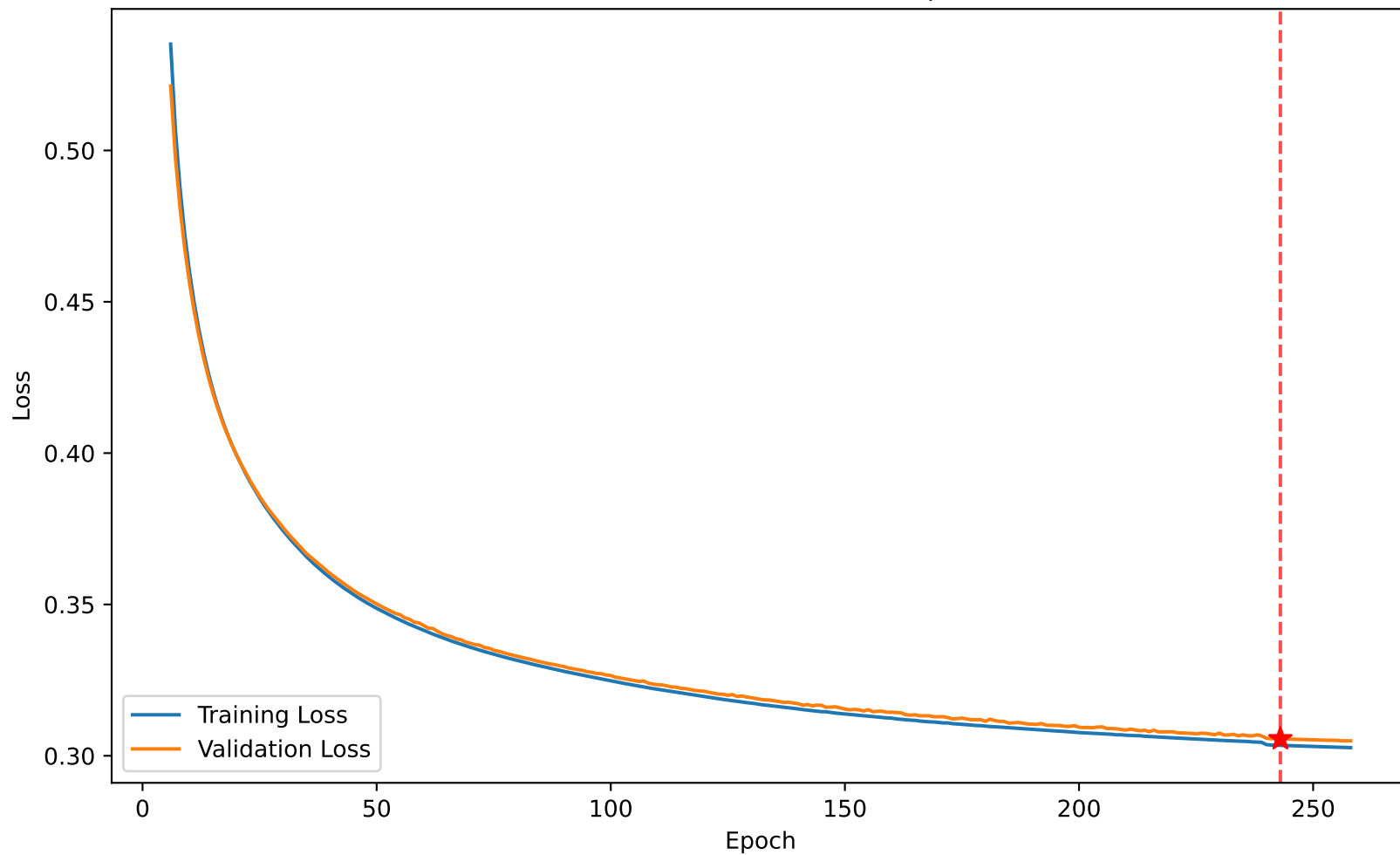
Loss 0.303 vs Val Loss 0.306 at epoch 243
