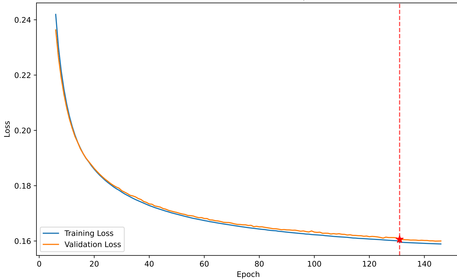
Loss 0.160 vs Val Loss 0.161 at epoch 131
